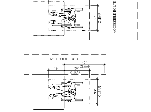
DINING ROOM SEATING CLEARANCES N.T.S. 8
