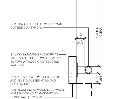
GRAB BAR 3/4" = 1'-0" 7
