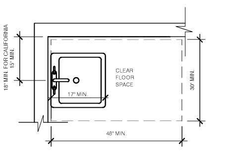
ACCESSIBLE LAVATORY 3/4" = 1'-0" 3
