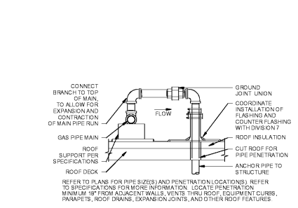
15 GAS PIPE ROOF PENETRATION NTS
