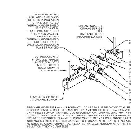
28 TRAPEZE PIPE HANGER NTS
