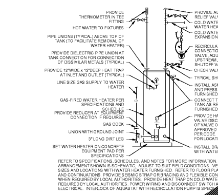
16 GAS FIRED WATER HEATER AND PUMP - FOR REFERENCE ONLY NTS
