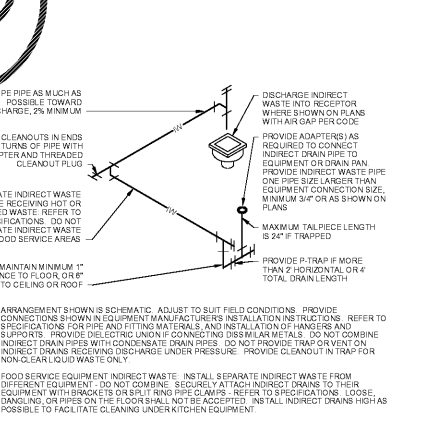
26 INDIRECT WASTE INSTALLATION - IPC NTS
