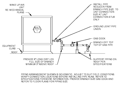
14 MAKE-UP AIR UNIT CONNECTIONS NTS
