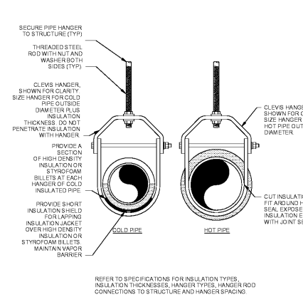
27 PIPE HANGER DETAIL NTS
