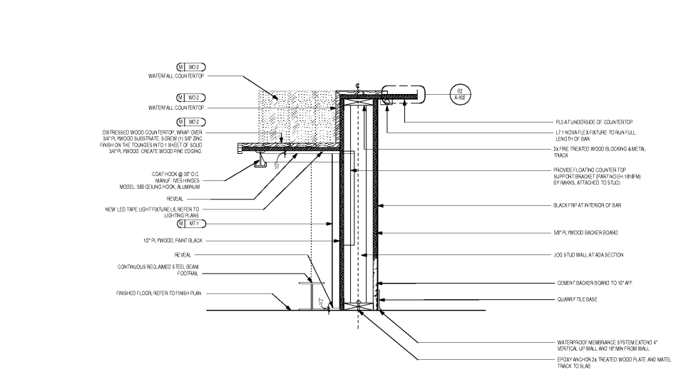
A2 BAR ADA - TYPICAL 1/8" = 1'-0"
