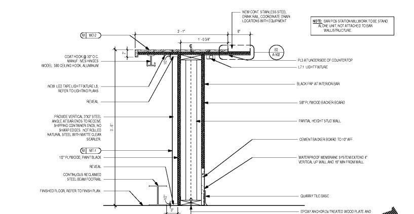
B1 BAR - TYP CONSTRUCTION 1/8" = 1'-0"
