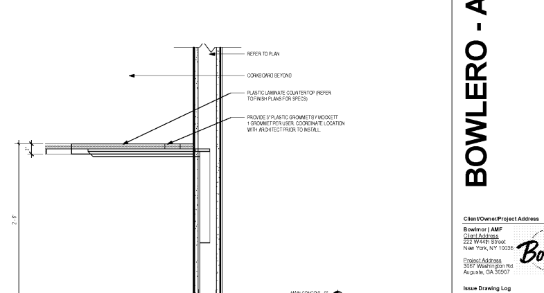
B3 OFFICE - DESK SECTION 1/8" = 1'-0"
