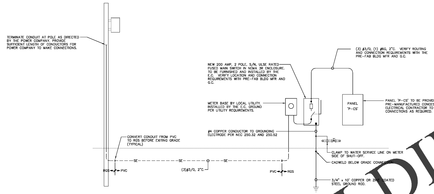
ELECTRICAL RISER DIAGRAM SCALE: NONE
