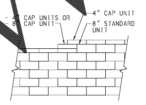
3 TOP OF WALL STEPS SCALE: 1/4" = 1'-0"
