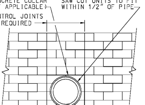
7 TYPICAL PIPE OUTLET DETAIL SCALE: 1/4" = 1'-0"
