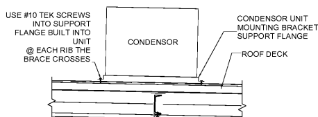
6 CONDENSER UNIT MOUNTING DETAIL M2 3/4" = 1'-0"
