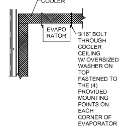
7 EVAPORATOR UNIT MOUNTING M2 3/4" = 1'-0"
