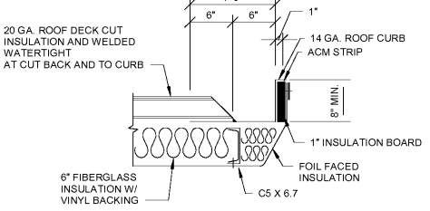
4 ROOF CURB DETAIL - PARTIAL M2 N.T.S.
