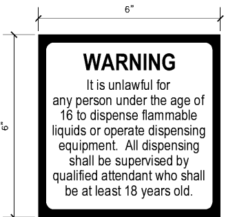
8 BLACK LETTERING WITH WHITE BACKGROUND SCALE: 6" = 1'-0"
