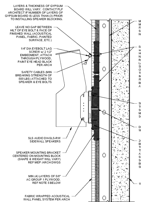
SPEAKER MOUNT @ EXISTING STUD WALL SECTION
