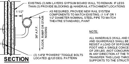
1 WALL MOUNT HANDRAIL DETAIL PLFS0.3 N.T.S.
