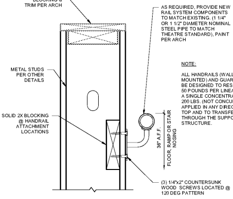
2 HANDRAIL @ NEW PARTITION WALL DETAIL PLFS0.3 N.T.S.
