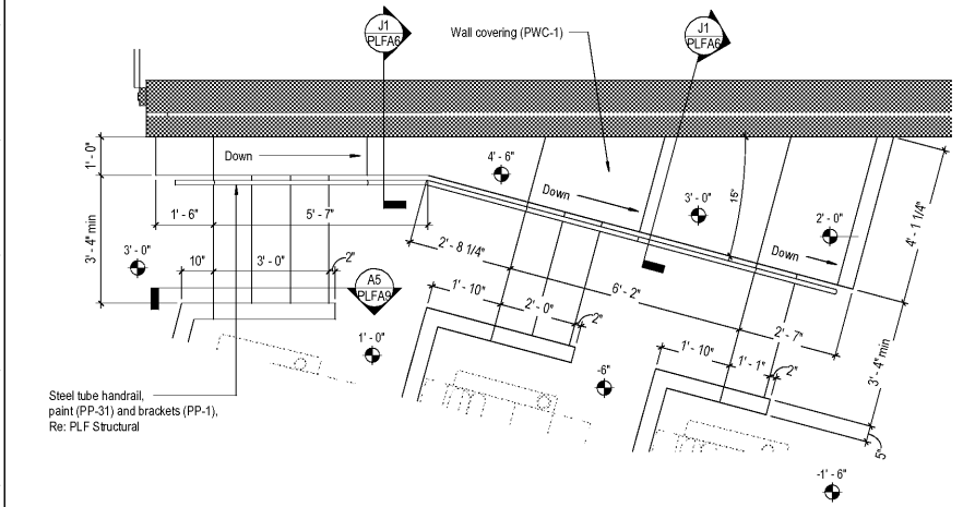
P1 Auditorium #1 - Buildout @ Front Steps PLFA1 1/2" = 1'-0"
