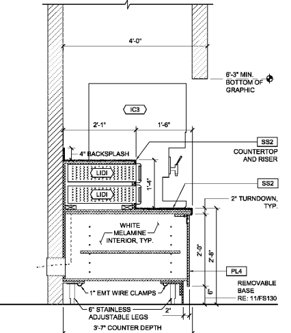
2 SECTION AT ICEE MACHINE SCALE: 3/4" = 1'-0"
