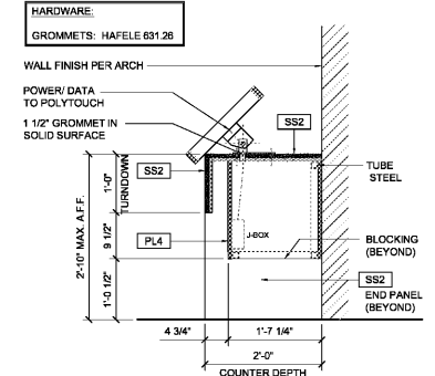
9 SECTION AT WALL SCALE: 3/4" = 1'-0"
