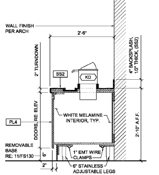
5 SECTION AT CONDIMENTS COUNTER SCALE: 3/4" = 1'-0"
