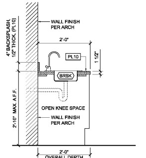
12 SECTION AT IN-COUNTER SINK SCALE: 3/4" = 1'-0"
