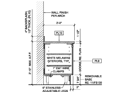
13 TYPICAL CASEWORK SECTION SCALE: 3/4" = 1'-0"
