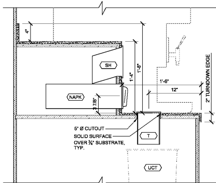
3 SECTION AT SELF-SERVE DRINKS SCALE: 1/2" = 1'-0"
