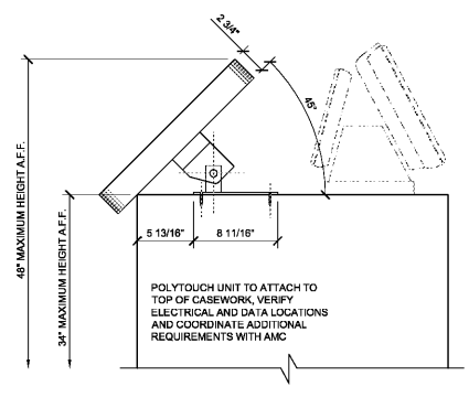
11 POLYTOUCH ATTACHMENT SECTION 1 1/2" = 1'-0"
