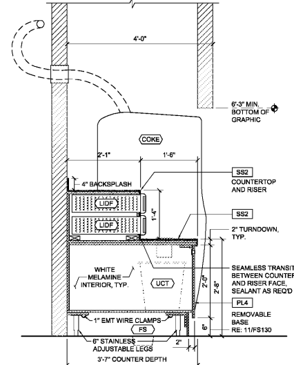
1 SECTION AT COKE MACHINE SCALE: 3/4" = 1'-0"
