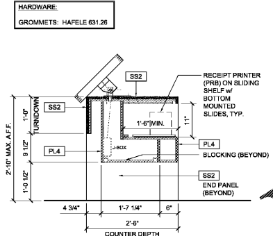
8 SECTION AT PRINTER SCALE: 3/4" = 1'-0"
