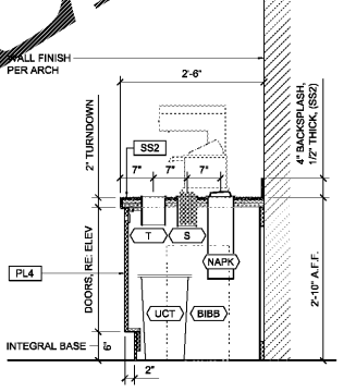
6 SECTION AT CONDIMENTS COUNTER SCALE: 3/4" = 1'-0"
