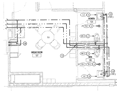
PARTIAL ENLARGED DOMESTIC WATER PLUMBING PLAN - EMPLOYEE USE RESTROOMS
