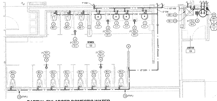
PARTIAL ENLARGED DOMESTIC WATER PLUMBING PLAN - PATRON USE WOMENS RESTROOMS
