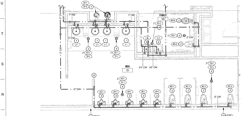
PARTIAL ENLARGED DOMESTIC WATER PLUMBING PLAN - PATRON USE MENS AND FAMILY RESTROOMS
