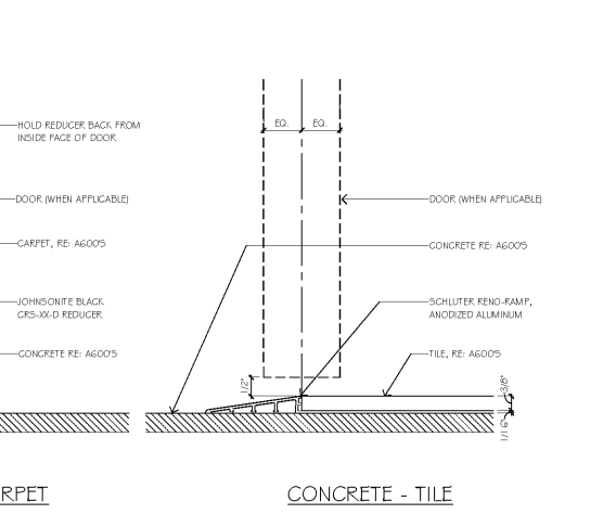
F8 FLOOR TRANSITION DETAILS 6" = 1'-0"
