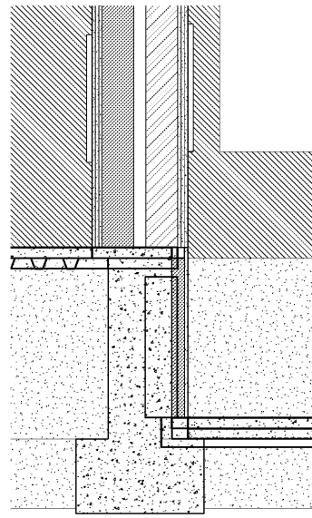
M4 SECTION AT SLAB OF AUDITORIUM #7 & #8 1" = 1'-0"
