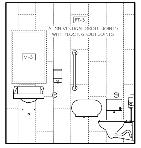
H5 RESTROOM ELEVATION - WOMEN (MEN MIRRORED) 1/2" = 1'-0"
