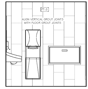
H16 RESTROOM ELEVATION - FAMILY 1/2" = 1'-0"
