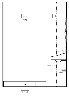
H1 RESTROOM ELEVATION - WOMEN (MEN MIRRORED) 1/2" = 1'-0"
