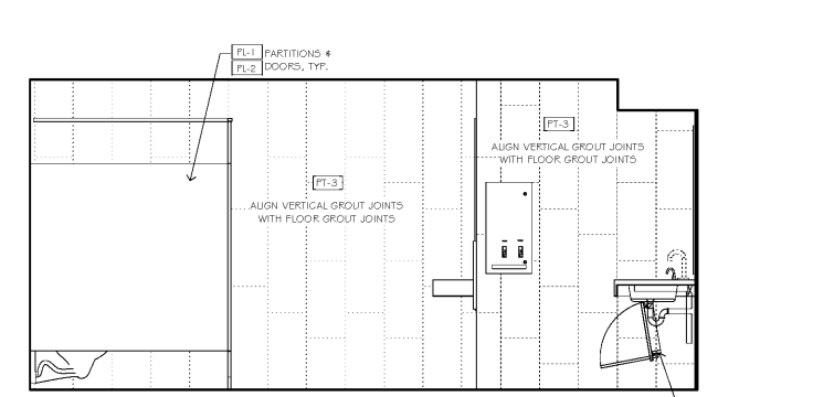
A12 RESTROOM ELEVATION - WOMENS
