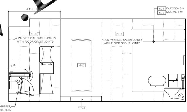
H12 RESTROOM ELEVATION - WOMENS
