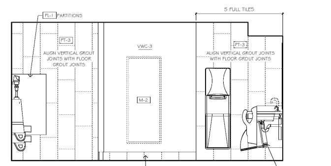
A12 RESTROOM ELEVATION - MENS
