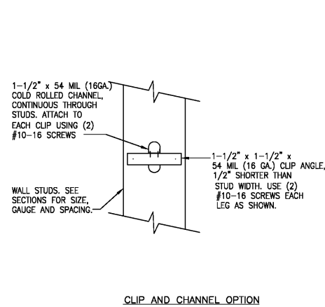
CLIP AND CHANNEL OPTION
