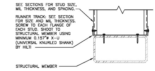
SECTION DETAIL: TRACK TO STRUCTURAL STEEL
