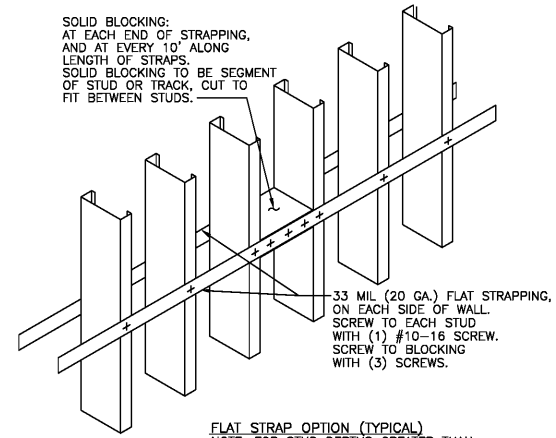
FLAT STRAP OPTION (TYPICAL) NOTE: FOR STUD DEPTHS GREATER THAN 6" THIS DETAIL MUST BE USED
