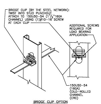
BRIDGE CLIP OPTION
