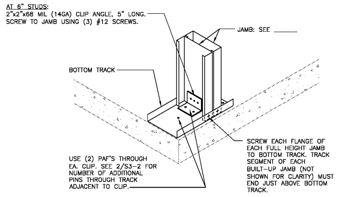
JAMB TO SLAB AT OPENINGS
