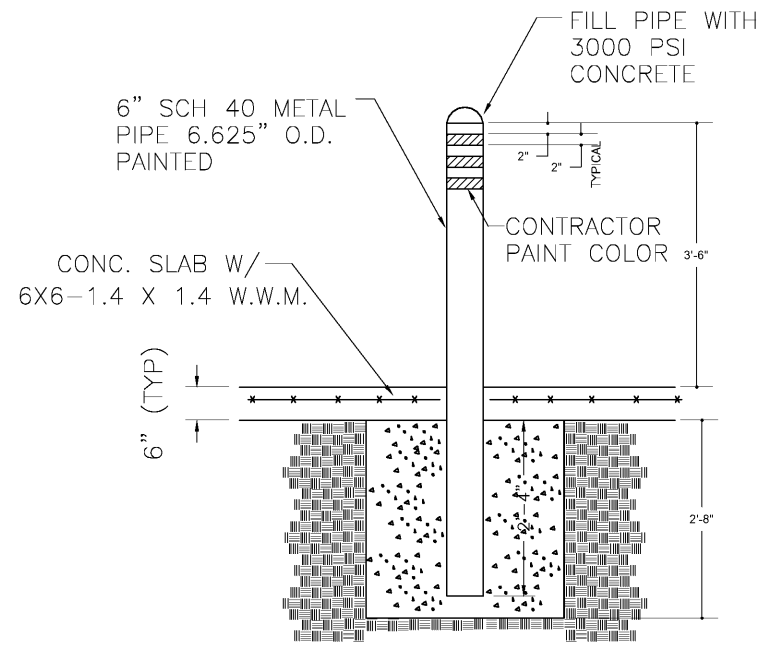
1 A9-2 BOLLARD DETAIL SCALE : 3/4" = 1'-0"
