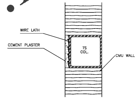
A A2-9 COLUMN DETAIL SCALE: 3" = 1'-0" USE WHERE COLUMN IS EXPOSED TO VIEW
