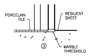
HEAD AND JAMB DETAILS AND DOOR SILL CONDITIONS SCALE: 1 1/2" = 1'-0"
