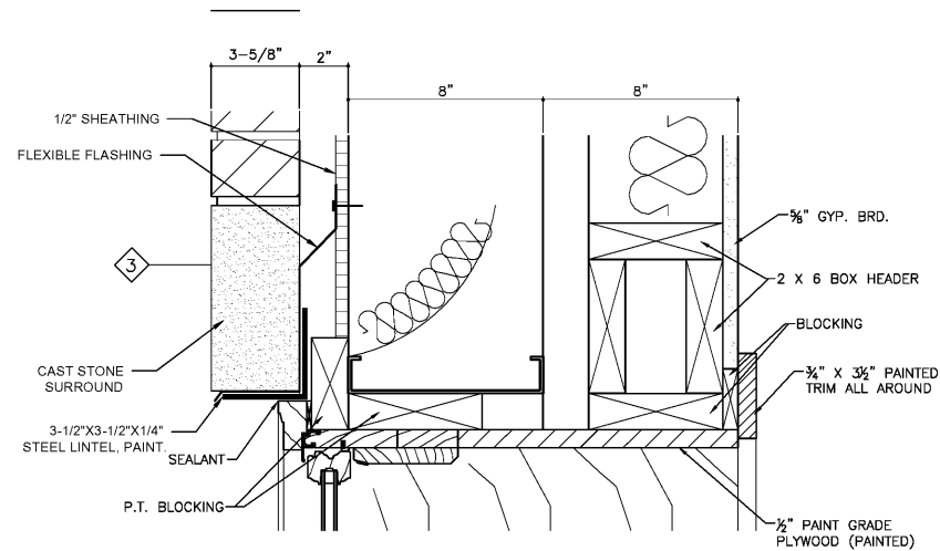
1 A2-9 HEAD - WINDOW SCALE: 3" = 1'-0" DOORS AND JAMB SIMILAR ADD. ALT. NO.2
