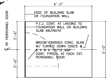
PLAN OF PERSONNEL DOOR CONCRETE "LANDING" SCALE: 1/2" = 1'-0"
