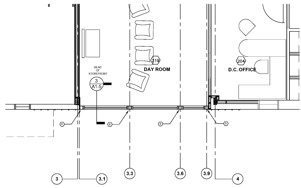
SECOND FLOOR DEDUCTIVE ALTERNATIVE NO.1 SCALE: 1/4" = 1'-0" DEDUCTIVE ALTERNATIVE NO.1 - TO OMIT WING WALL AND ALL GLASS 2-STORY ENTRY
