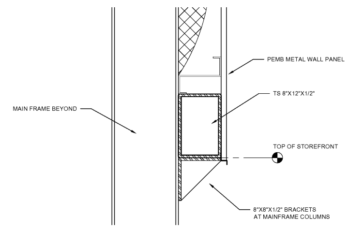
STOREFRONT HEAD DEDUCTIVE ALTERNATIVE NO.1 SCALE: 1/4" = 1'-0" DEDUCTIVE ALTERNATIVE NO.1 - TO OMIT WING WALL AND ALL GLASS 2-STORY ENTRY
