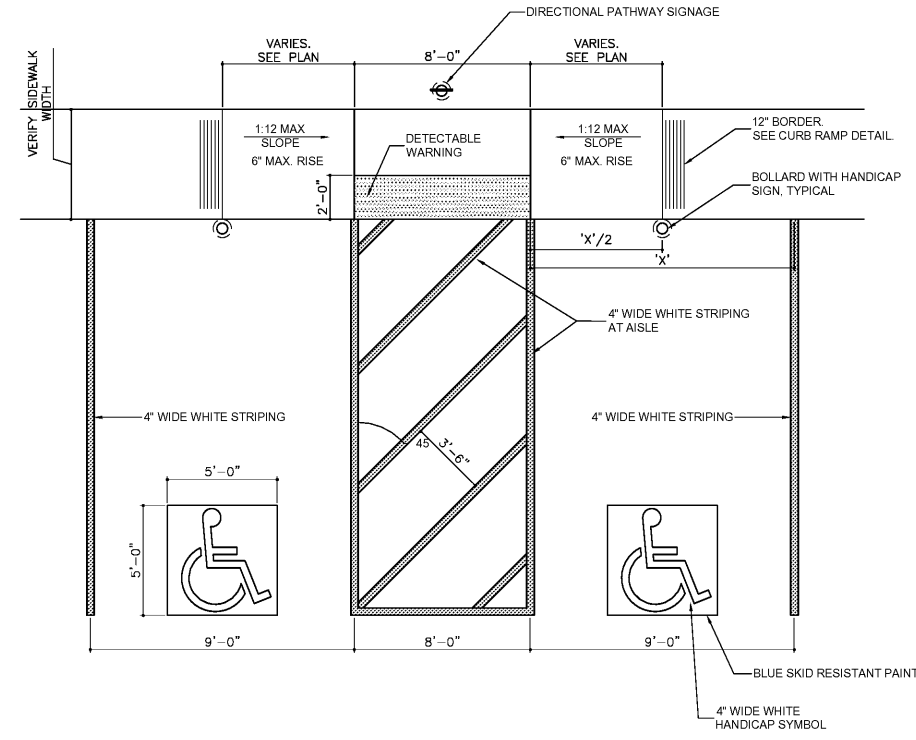
4 SD-4 TYPICAL ACCESSIBLE PARKING DETAIL SCALE: 1/4\"/>
