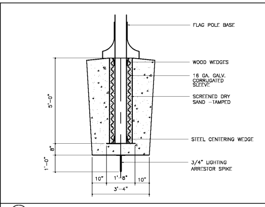
1 SD-4 FLAGPOLE DETAIL NO SCALE LOCATE AS DIRECTED BY ARCHITECT
