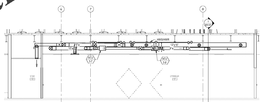
3 MECHANICAL SECTION 1/4" = 1'-0"
