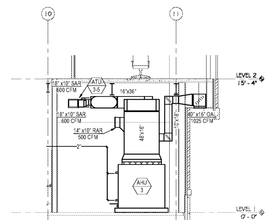
4 MECHANICAL SECTION 1/4" = 1'-0"
