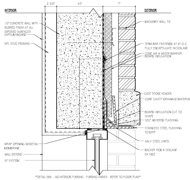
G1 TYP WIN HEAD - C.I.P. & BRICK SCALE: 3" = 1'-0"
