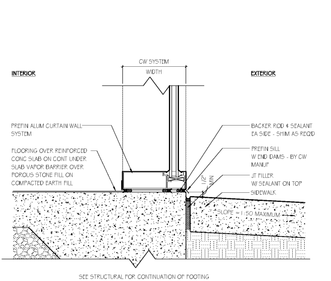
A6 EXT CURTAIN WALL @ SIDEWALK SCALE: 3" = 1'-0"
