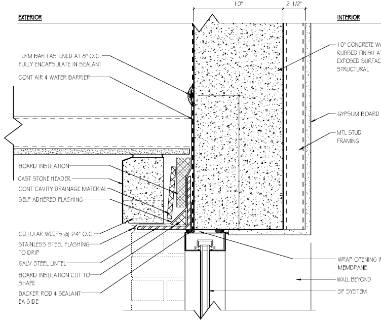
G6 WIN HEAD @ CANTILEVER SCALE: 3" = 1'-0"
