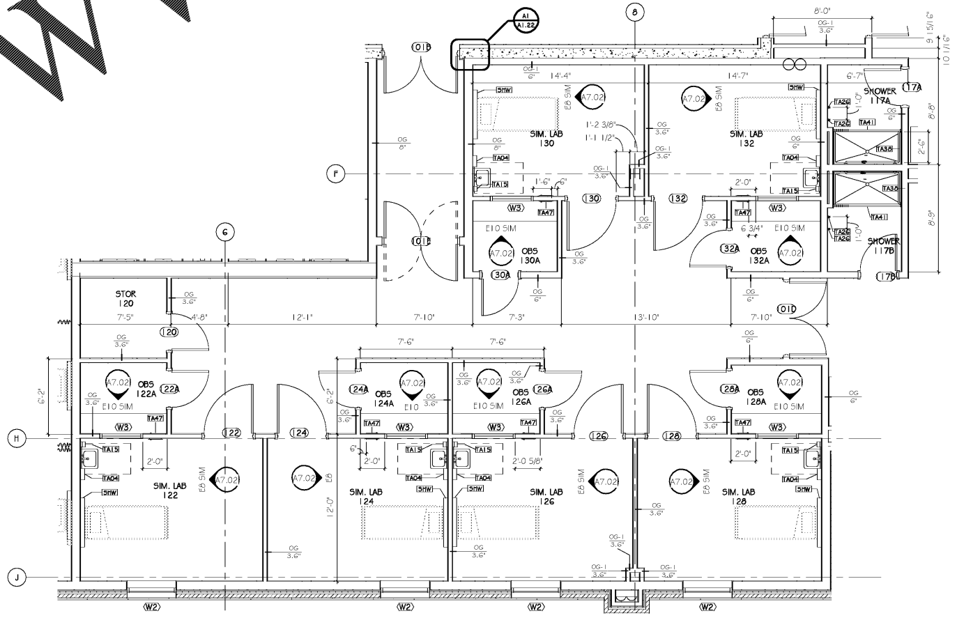
A6 SIMULATION LAB SCALE: 1/4" = 1'-0"
