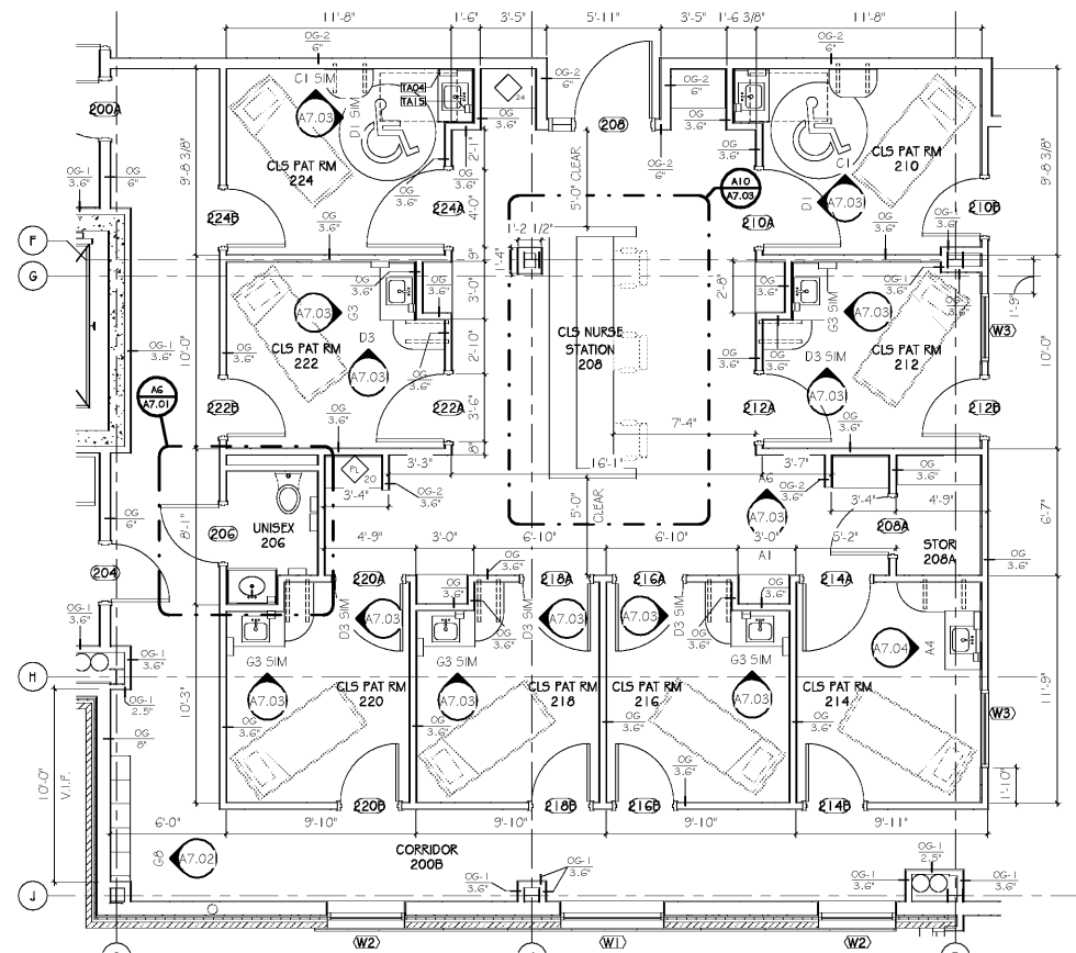
F1 CLINICAL SIM PATIENT ROOMS SCALE: 1/4" = 1'-0"
