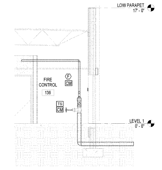
WATER PIPE ENTRY ELEVATION 1/4" = 1'-0"
