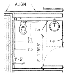
B2 ENLARGED TOILET - MEN 1/4" = 1'-0"
