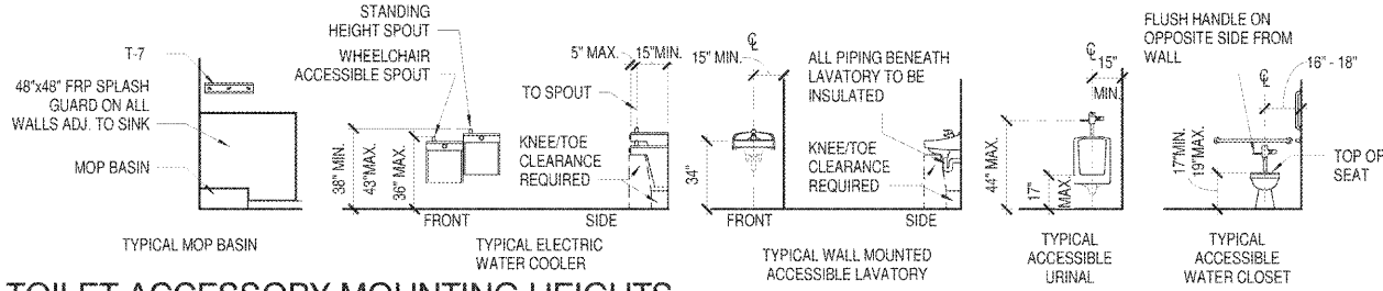
C1 TOILET ACCESSORY MOUNTING HEIGHTS 1/4" = 1'-0"
