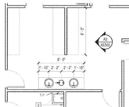
A3 ENLARGED - WEAPONS CLEANING RM 1/4" = 1'-0"
