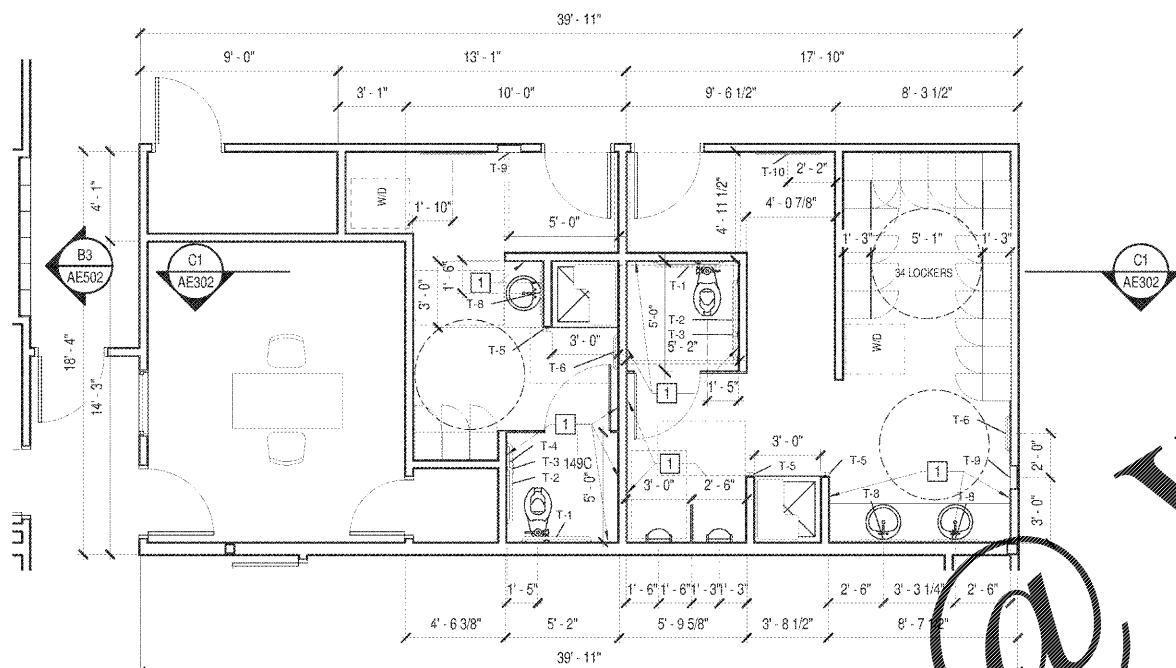
B1 ENLARGED FLOOR PLAN - POLICE LOCKERS 1/4" = 1'-0"
