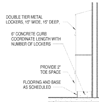
C3 LOCKER DETAIL 1/2" = 1'-0"
