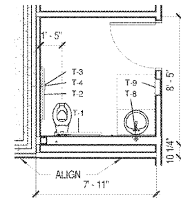
B3 ENLARGED TOILET - WOMEN 1/4" = 1'-0"
