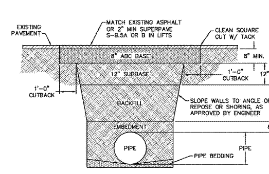
WD-9 DOUBLE SERVICE CONNECTION NOT TO SCALE
