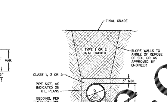
WD-14 PAVEMENT REPAIR WHERE PIPE IS INSTALLED NOT TO SCALE
