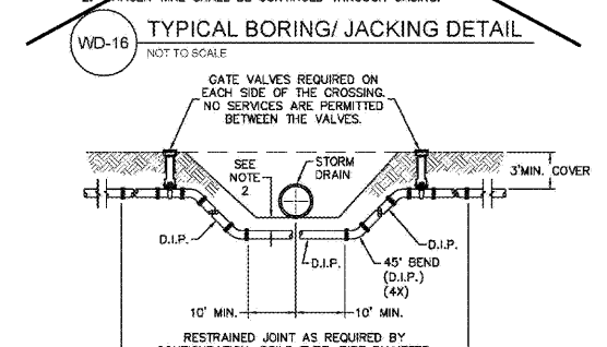
WD-16 TYPICAL BORING/JACKING DETAIL NOT TO SCALE
