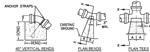
WD-4 THRUST BLOCK DETAIL NOT TO SCALE
