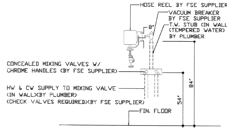
1 TYPICAL HOSE REEL DETAIL K301 NOT TO SCALE
