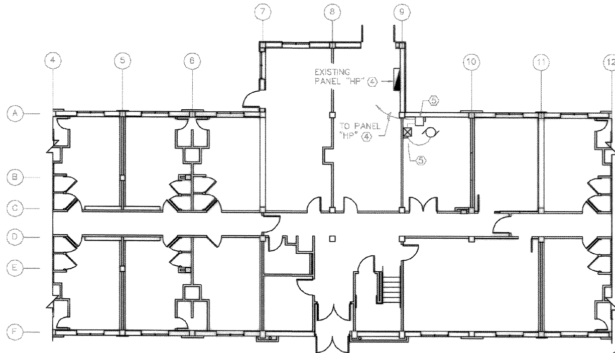
ELECTRICAL FIRST FLOOR PLAN - BUILDING 475 (CHILLER PLANT REPLACEMENT OPTION) SCALE: 1/8" = 1'-0"
