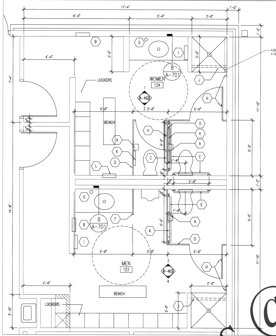
1 ENLARGED TOILET PLAN - #123, #124 1/2"=1'-0"
