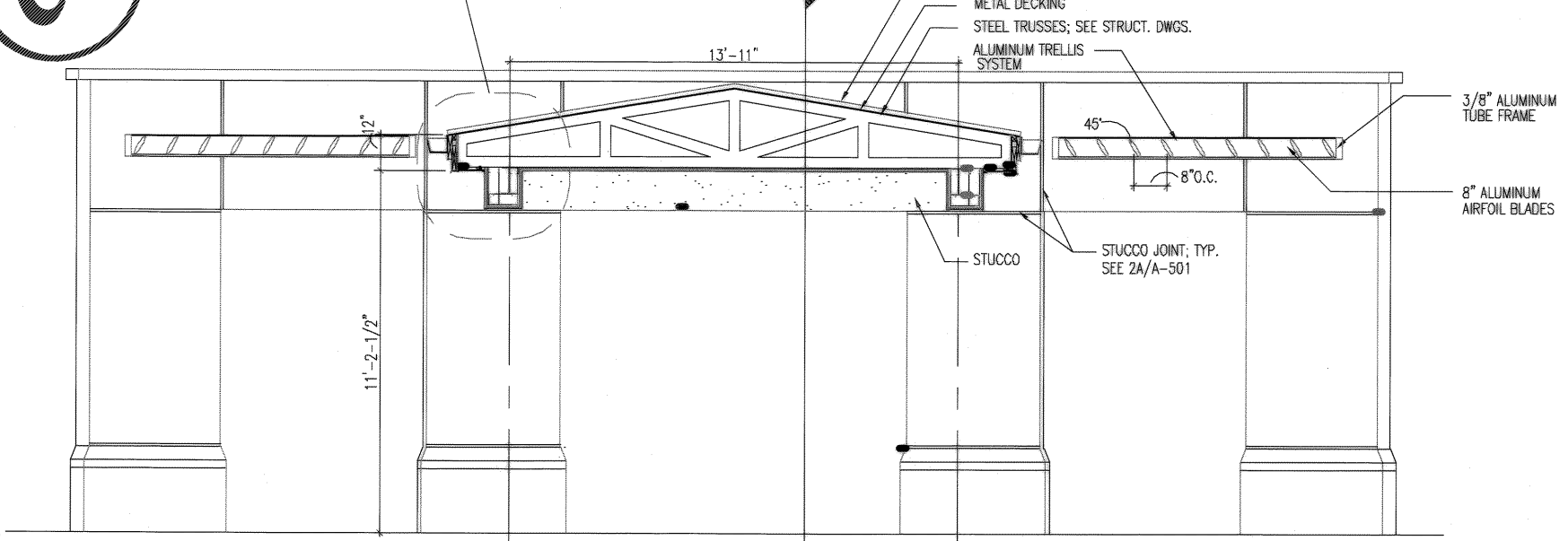
3 WALL SECTION 3/8"=1'-0"
