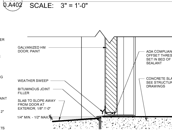
S3 0.A402 SILL FOR EXTERIOR DOOR AT EXTERIOR WALL SCALE: 3" = 1'-0"
