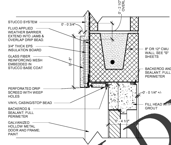
H4 0.A402 HEAD FOR HM DOOR AT EXTERIOR STUCCO WALL SCALE: 3" = 1'-0"
