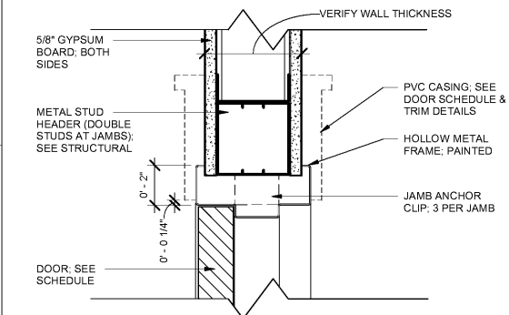
H1/J1 0.A402 HEAD/JAMB FOR INTERIOR HM FRAME DOOR SCALE: 3" = 1'-0"
