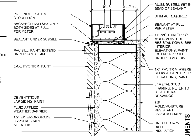
S4 0.A402 SILL FOR ALUM. STOREFRONT AT CEMENTITIOUS SIDING SCALE: 3" = 1'-0"
