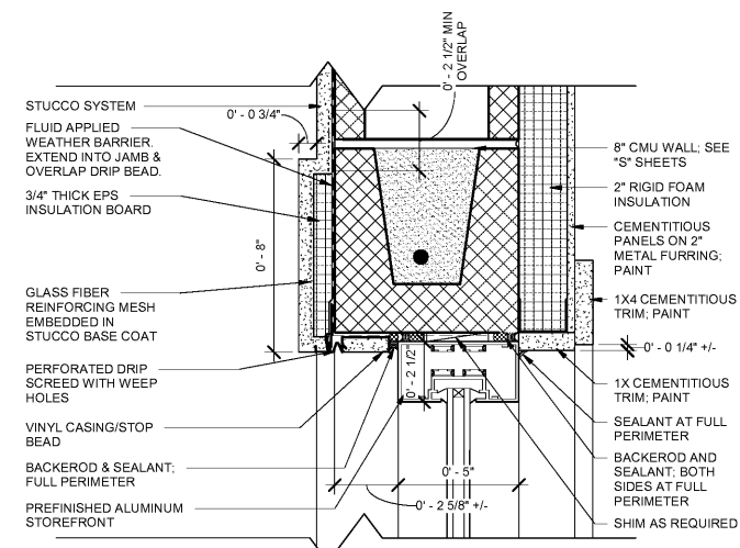
H3 0.A402 HEAD FOR ALUM. STOREFRONT AT CMU STUCCO WALL SCALE: 3" = 1'-0"
