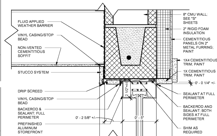
H2 0.A402 HEAD FOR ALUM. STOREFRONT RENTAL WINDOW AT DOCK HOUSE SCALE: 3" = 1'-0"
