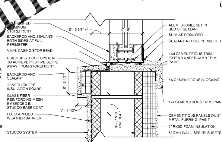
S2 0.A402 SILL FOR ALUM. STOREFRONT AT EXT. STUCCO DOCK HOUSE WALL SCALE: 3" = 1'-0"
