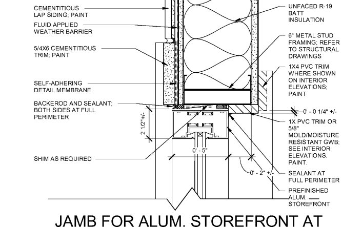
J4 0.A402 JAMB FOR ALUM. STOREFRONT AT CEMENTITIOUS SIDING SCALE: 3" = 1'-0"
