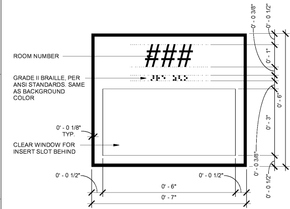
G1 Q.A004 TYP. SIGNAGE MOUNTING ELEV SCALE: 3/8" = 1'-0"
