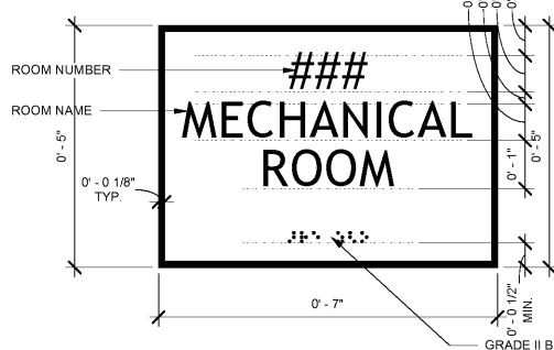
E3 Q.A004 SIGN TYPE B - TYPICAL PANEL WALL SIGN SCALE: 6" = 1'-0"
