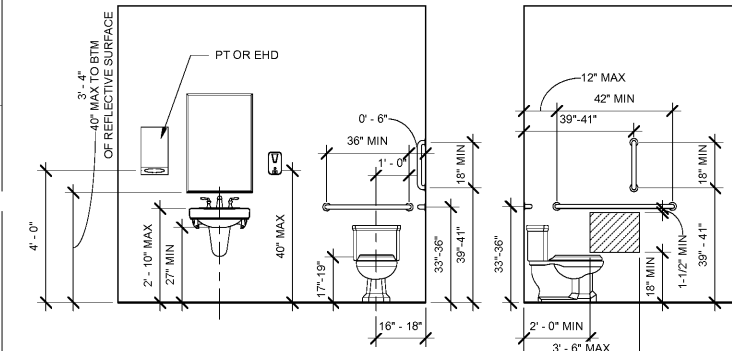
C1 Q.A004 TYP. ADA TOILET ELEVATIONS SCALE: 3/8" = 1'-0"
