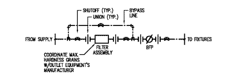
3 WATER FILTER DETAIL NOTE
