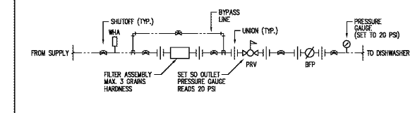
4 DISHWASHER CONNECTION DETAIL NOTE
