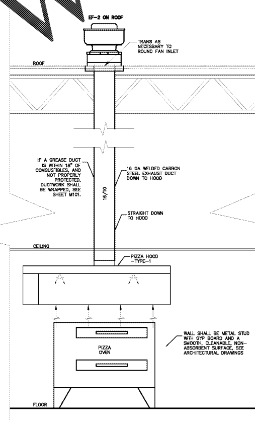
4 PIZZA HOOD FRONT VIEW M508 SCALE: NONE
