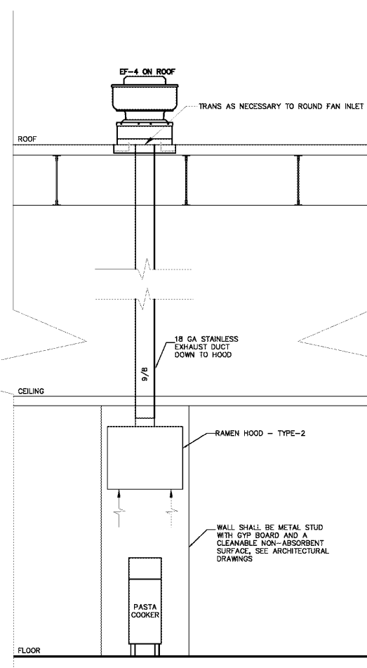
1 RAMEN HOOD FRONT VIEW M508 SCALE: NONE
