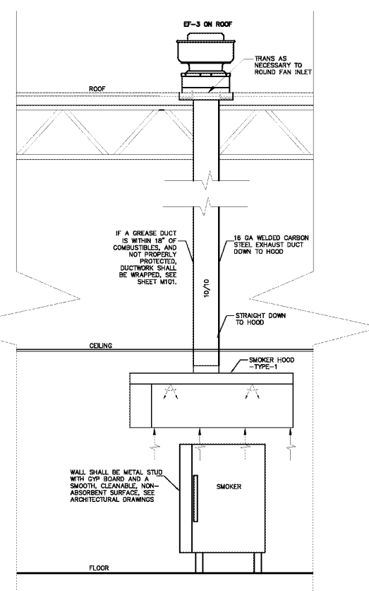
5 SMOKER HOOD FRONT VIEW M508 SCALE: NONE
