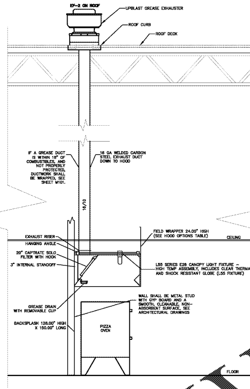
2 PIZZA HOOD SIDE VIEW M507 SCALE: NONE
