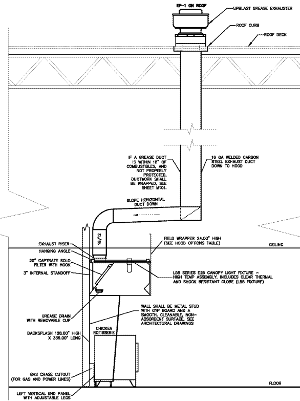
1 COOKLINE HOOD SIDE VIEW M507 SCALE: NONE
