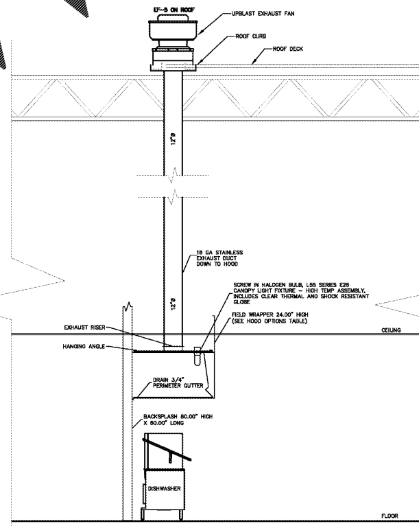
5 DISHWASHER HOOD SIDE VIEW M507 SCALE: NONE
