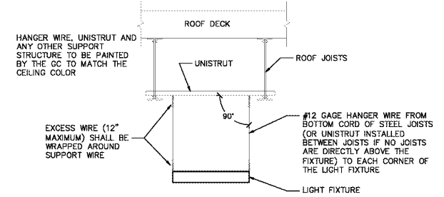
3 LIGHTING SUPPORT DETAIL E201 NOT TO SCALE
