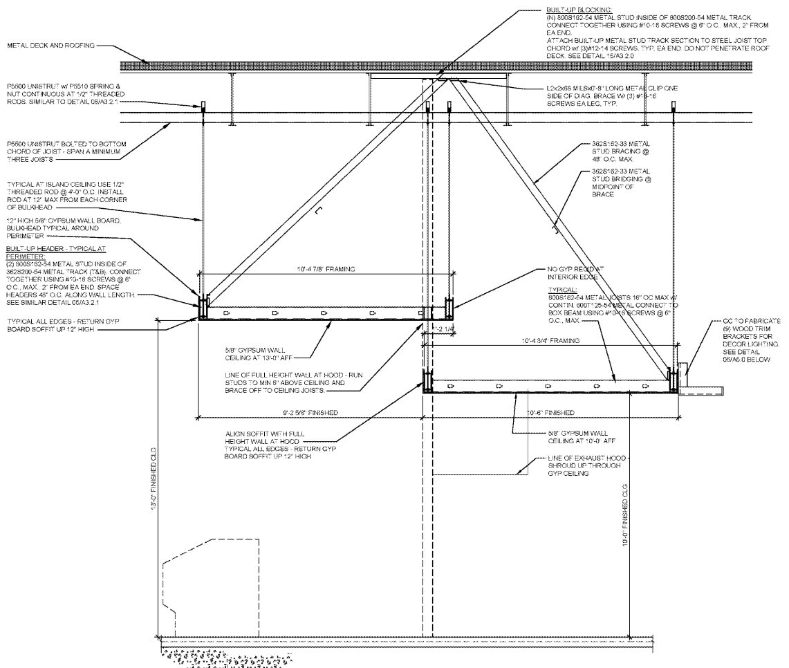
01 GRAB-n-GO ISLAND CEILING SCALE: 1/2" = 1'-0"
