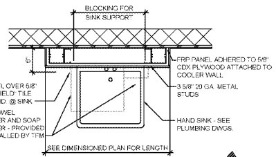
10 HAND SINK PLAN DETAIL SCALE: 1" = 1'-0"
