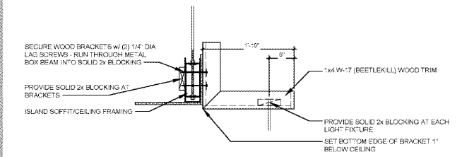
05 DECOR LIGHTING BRACKET DETAIL SCALE: nts
