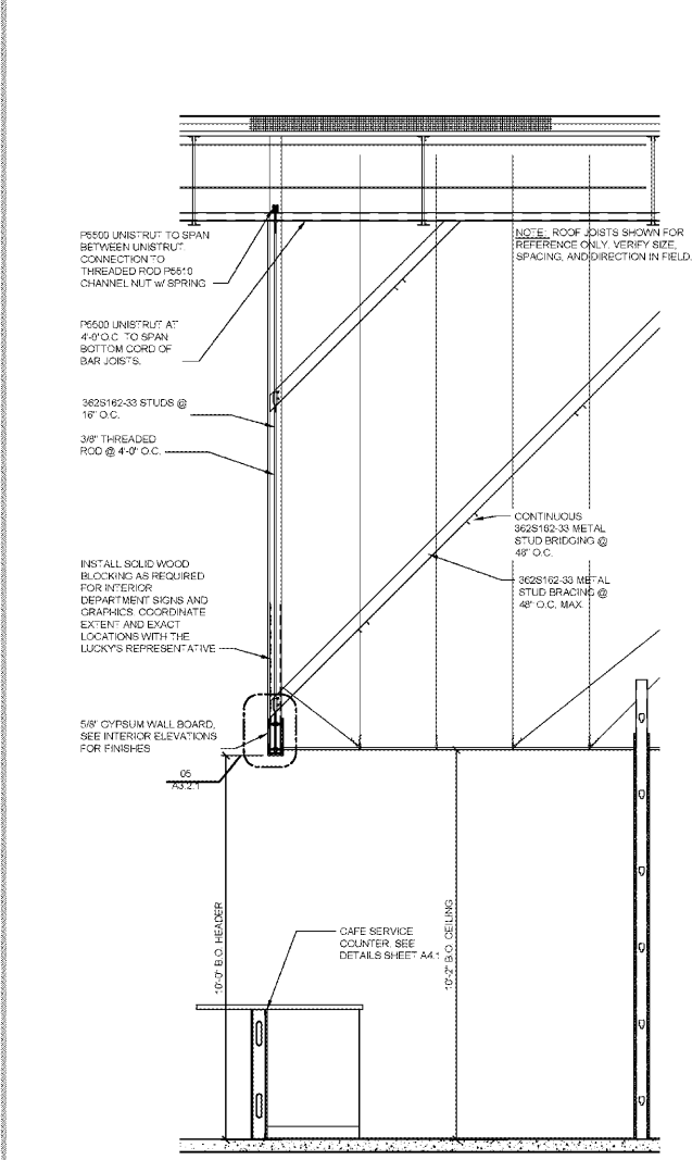
03 SECTION AT CAFE SCALE: 1/2" = 1'-0"
