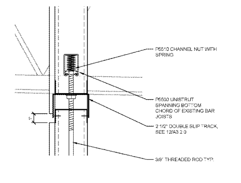
08 UNISTRUT CONNECTION TO JOIST SCALE: 3" = 1'-0"
