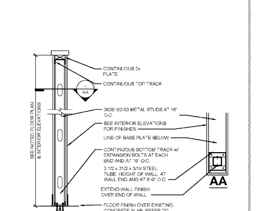
07 TYPICAL LOW WALL FRAMING SCALE: 1" = 1'-0"
