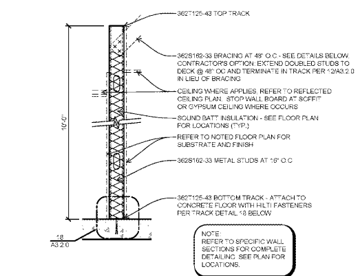
01 WALL TYPE - 3 5/8" PARTIAL HEIGHT SCALE: 1" = 1'-0"
