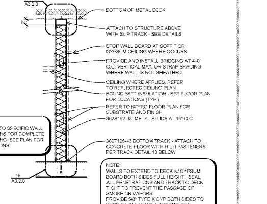
03 WALL TYPE - 3 5/8" TO STRUCTURE SCALE: 1" = 1'-0"
