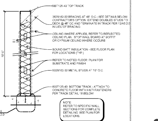
04 WALL TYPE - 6" PARTIAL HEIGHT INSUL. SCALE: 1" = 1'-0"
