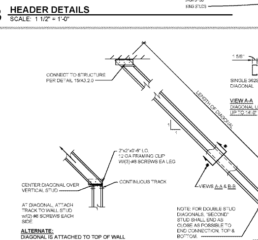
17 DIAGONAL BRACING DETAIL SCALE: 1" = 1'-0"
