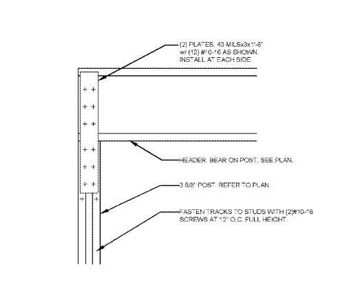
11 BEAM TO POST CONNECTION SCALE: 1 1/2" = 1'-0"
