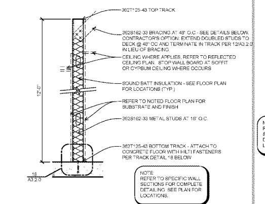
02 WALL TYPE - 3 5/8" PARTIAL HEIGHT SCALE: 1" = 1'-0"
