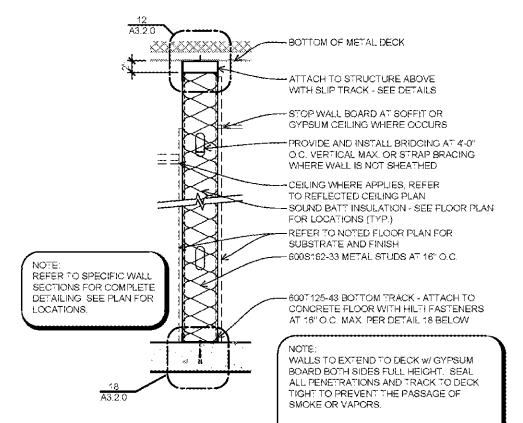
06 WALL TYPE - 6" TO STRUCTURE SCALE: 1" = 1'-0"
