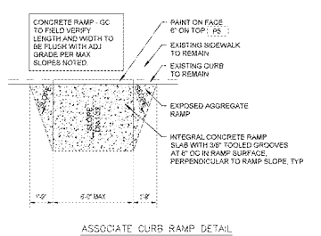
ASSOCIATE CURB RAMP DETAIL
