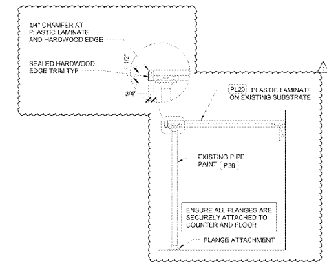
2 COUNTER SECTION 1" = 1'-0"
