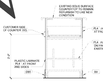
5A BASE CABINET SECTIONS 1" = 1'-0"
