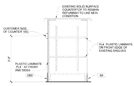
5 BASE CABINET SECTIONS 1" = 1'-0"
