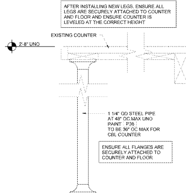
1 COUNTER LEG 3/8" = 1'-0"
