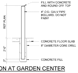
11 GARDEN CENTER/INTERIOR BOLLARD DETAIL 1/2" x 1'-0"
