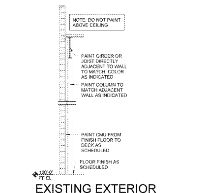
2 EXISTING EXTERIOR CMU WALL SECTION 1/4" x 1'-0"
