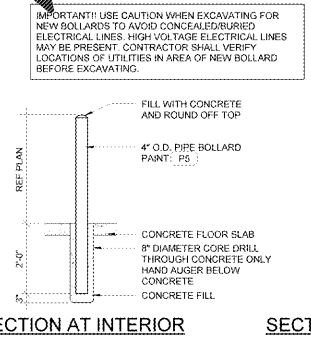
11 GARDEN CENTER/INTERIOR BOLLARD DETAIL 1/2" x 1'-0"
