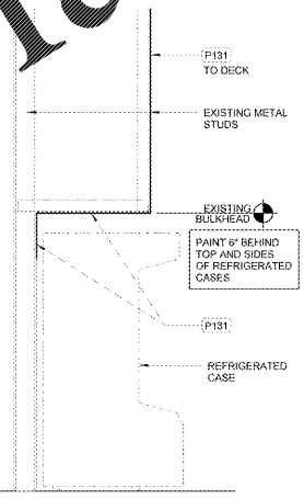
5 BULKHEAD AT CASE 1/2" x 1'-0"
