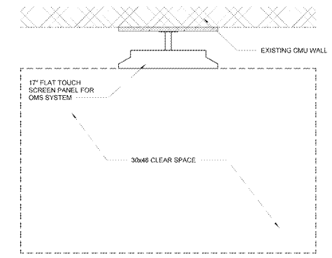
21 ORDER MANAGEMENT SYSTEM (OMS) WALL BLOCKING PLAN 1 1/2" x 1'-0"
