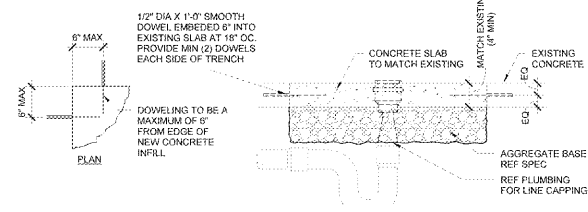
15 SLAB REPLACEMENT DETAIL 3/4" x 1'-0"
