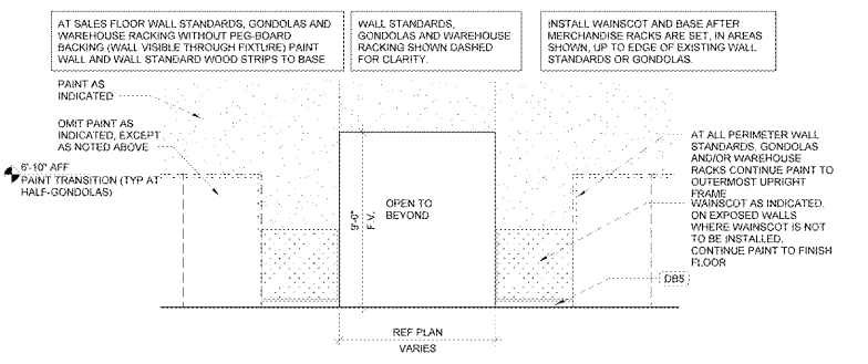
3 SALES WALL FINISHES AT PERIMETER HALF-GONDOLAS 3/4" x 1'-0"
