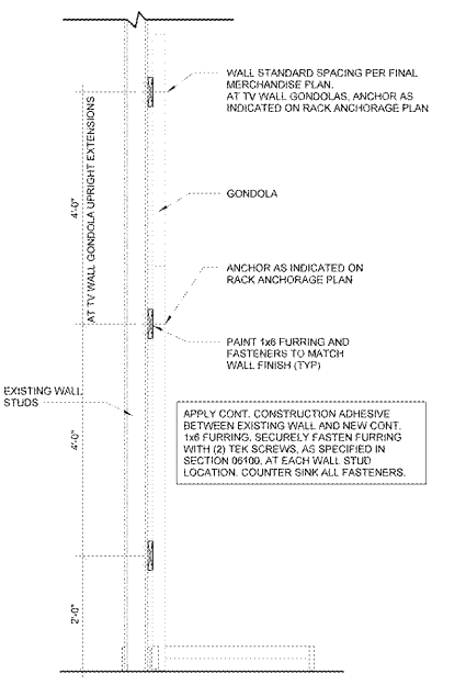
9 GONDOLA ANCHORING ON STUD WALL 3/4" x 1'-0"
