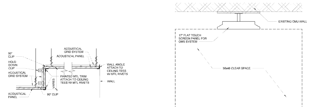
22 CEILING SECTION 1 1/2" x 1'-0"
