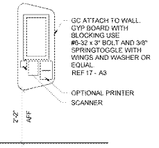
19 IN STORE MOUNTED KIOSK ELEVATION 1/2" x 1'-0"
