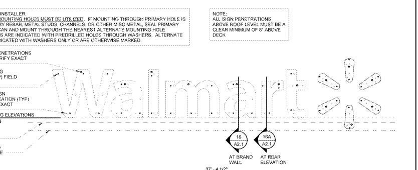
1 5'-6" WALMART SIGN 1/4" x 1'-0"
