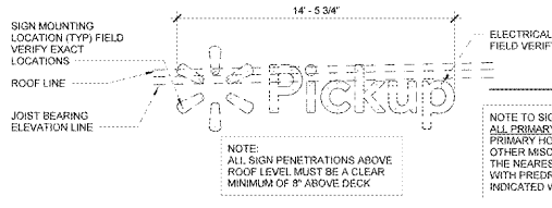
3 PICKUP SIGN MOUNTING DIAGRAM 2'-6" 1/4" x 1'-0"
