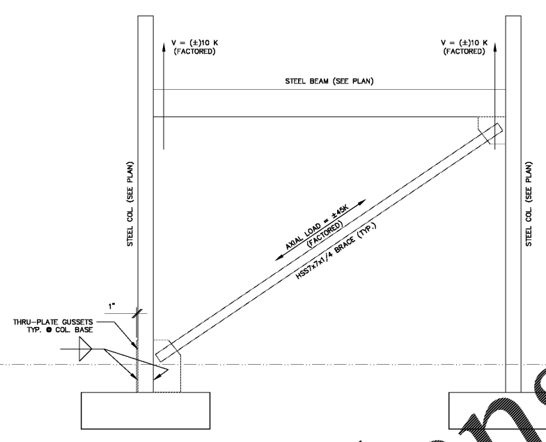
TYPICAL SINGLE BAY BRACED FRAME
