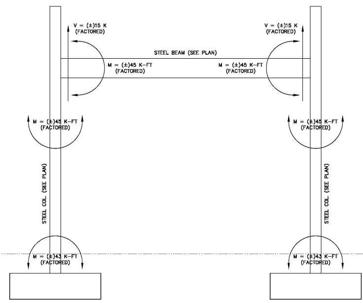
TYPICAL SINGLE BAY MOMENT FRAME
