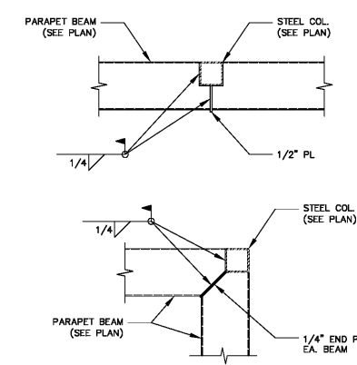
TYPICAL PARAPET CONNECTIONS (PLAN VIEW)
