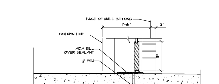
10 EXTERIOR WALL AT DOOR SILL 1 1/2" x 1'-0"
