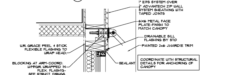
2 HEAD DETAIL 1 1/2" x 1'-0"
