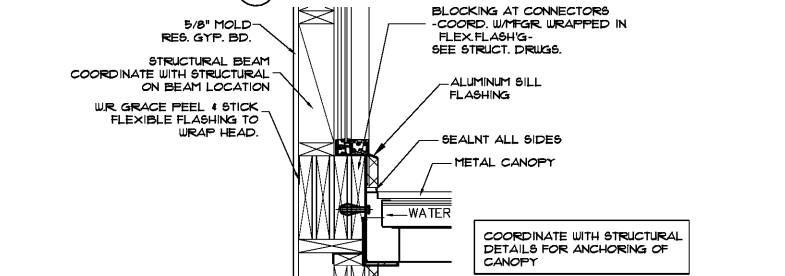
3 SILL DETAIL 1 1/2" x 1'-0"
