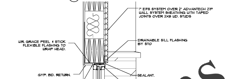
4 HEAD DETAIL 1 1/2" x 1'-0"
