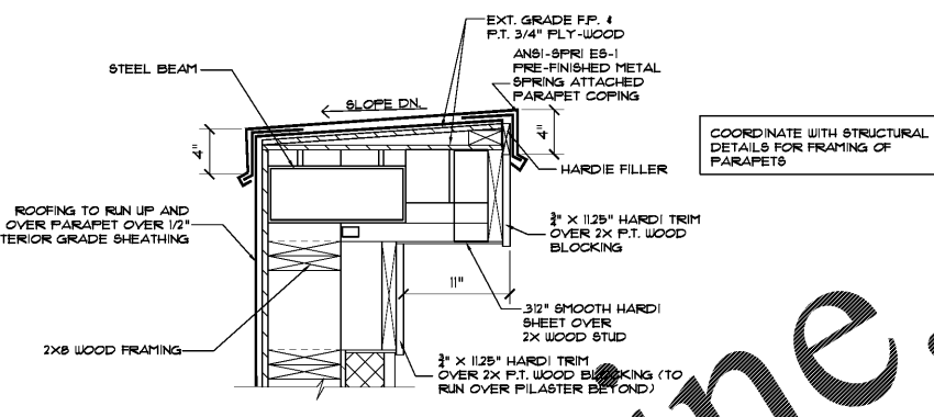
12 PARAPET DETAIL 1 1/2" x 1'-0" STEEL PARAPET
