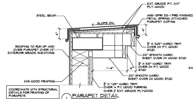
1 PARAPET DETAIL 1 1/2" x 1'-0"
