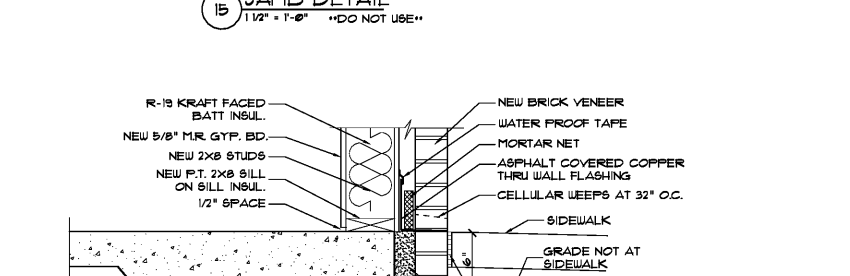
11 FOUNDATION AT NEW CONST. 1 1/2" x 1'-0"
