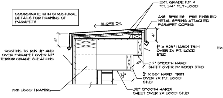
6 PARAPET DETAIL 1 1/2" x 1'-0" WOOD PARAPET
