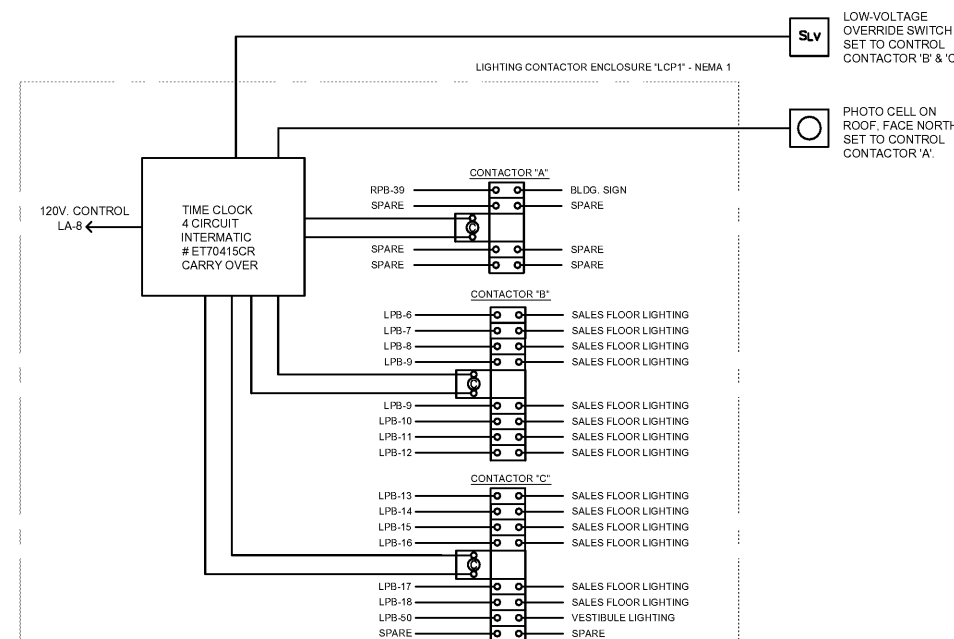
LIGHTING CONTROL DIAGRAM - "LCP-B"
