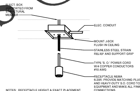
DROP CORD DETAIL
