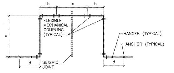
B3 PIPING CROSSING A SEISMIC JOINT DETAIL "A" SCALE: NONE
