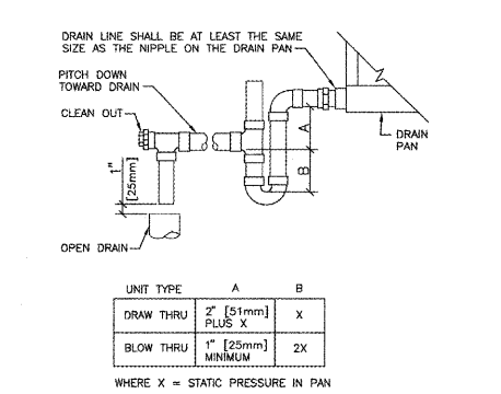
F9 AIR HANDLING UNIT DRAIN TRAP DETAIL SCALE: NONE
