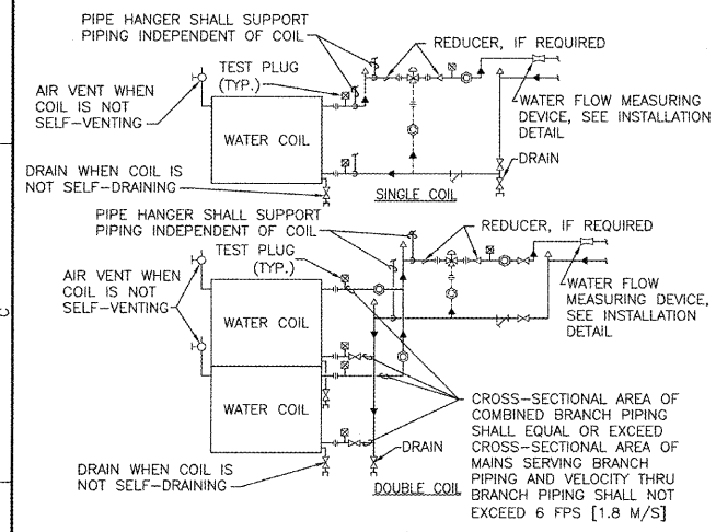
E1 TYPICAL CONNECTIONS TO WATER COIL SCALE: NONE
