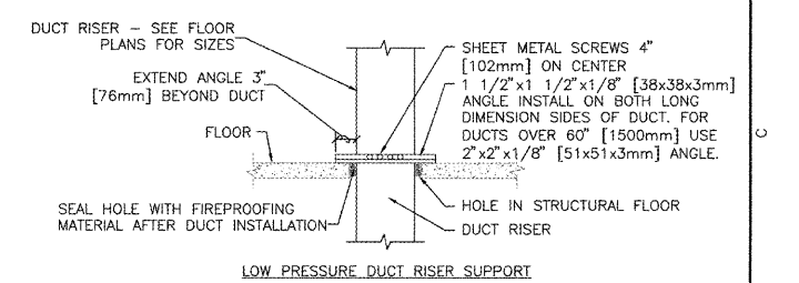
D9 LOW, MEDIUM AND HIGH PRESSURE DUCT RISER SUPPORTS SCALE: NONE
