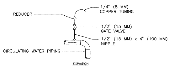
E6 TYPICAL CHILLED AND HOT WATER PIPING DRAIN VALVE CONNECTIONS SCALE: NONE
