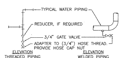
E6 TYPICAL CHILLED AND HOT WATER PIPING DRAIN VALVE CONNECTIONS SCALE: NONE
