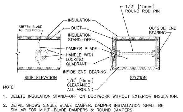
B1 VOLUME DAMPER DETAIL SCALE: NONE
