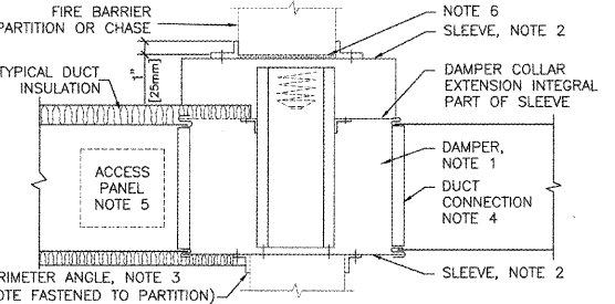
D3 SECTION THRU TYPICAL FIRE DAMPER INSTALLATION SCALE: NONE
