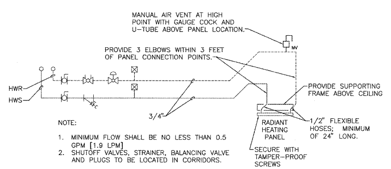
B6 HYDRONIC RADIANT CEILING PANELS - PIPING CONNECTIONS SCALE: NONE
